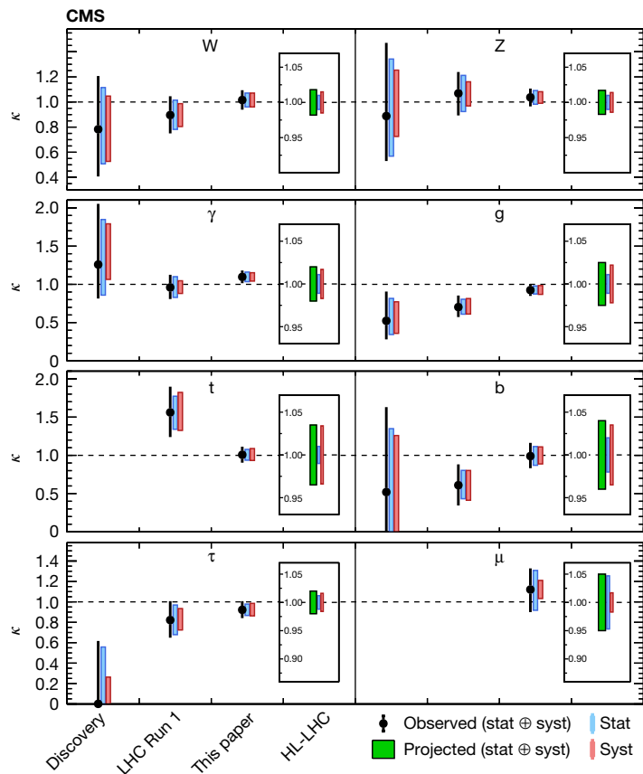
using the full data from LHC Run 1, in the dataset used in this paper and the expected 1-s.d. uncertainty at the HL-LHC for \mathcal{L} = 3,000 \text{ fb}^{-1} . The H \rightarrow \mu\mu and \kappa measurements were not available for earlier datasets owing to the lack of sensitivity.
