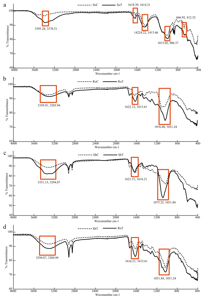
Figure 4. FTIR spectra for soil (a) and T. qataranse root and foliar (b–d). (a) Soil control (SoC) vs Soil treatment (SoT). (b) Root control (RoC) vs Root treatment (RoT). (c) Soot control (ShC) Shoot treatment (ShT). (d) Root treatment (RoT) vs Shoot treatment (ShT).
