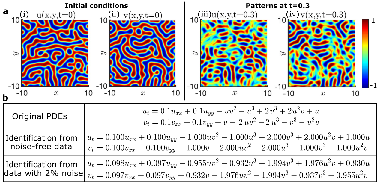
Figure 5. Demonstration of data-driven discovery of PDEs with ATSBLL using a reaction–diffusion system. (a–i,ii) Snapshots of the initial conditions for the variables u and v , respectively. (a–iii,iv) u and v at time t = 0.3 . (b) The table shows the original PDEs for the reaction–diffusion system and the identified PDEs for noise-free data and data with 2% Gaussian noise. Inference is conducted with a library containing 35 terms. The numerical calculations are done with a time step \Delta t = 0.0034 in the time interval t = [0, 0.6] . The space domain has size 20 \times 20 and is covered with a 256 \times 256 grid with periodic boundary conditions.
