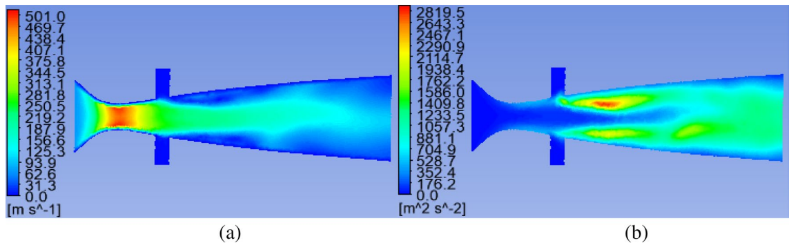
Figure 3. Internal cloud map of supersonic nozzle. (a) Velocity cloud map. (b) Turbulent kinetic energy cloud map.
