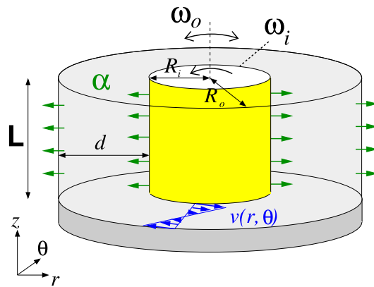
Figure 1. Schematics of the Taylor–Couette system, illustrating radial flow in a counter-rotating configuration, including a sketch of the laminar velocity profile, v(r, \theta) (not to scale). The radial flow can be outward, ( \alpha > 0 ) (as shown), or inward, ( \alpha < 0 ). Only the bottom lid serving as one of the axial end walls is indicated (dark gray).
