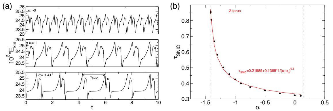
Figure 15. Saddle node on an invariant circle bifurcation for pV_1 . (a) Time series of E_{kin} for pV_1 at \alpha as indicated; (b) Variation of \tau_{SNIC} with \alpha for pV_1 (see Fig. 14). The solid circles are the computed periods, and the line is a fit of the form, \tau_{SNIC} = a_0 + a_i/\sqrt{\alpha - \alpha_c} . Note that in the region, 0.15 < \alpha < 0.67 , no pV state, whether stable nor unstable, can be detected, even in subspaces (see section “Unstable pV states”).
