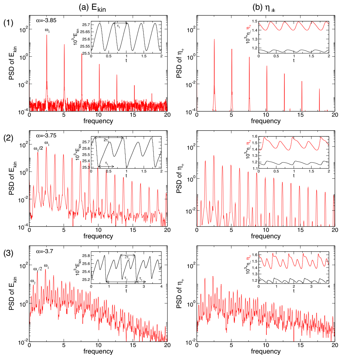
Figure 6. Time series and power spectral densities (PSDs) of the pulsating flow twin-pair state, T_2^{\text{puls}} , for different \alpha . PSDs of (a) E_{\text{kin}} and (b) \eta_{\pm} for: (1) T_2^{\text{puls}} at \alpha = -3.85 with pulsating time \tau_1 \approx 0.197 with corresponding frequency \omega_1 \approx 2.532 ; (2) T_2^{\text{puls}} at \alpha = -3.75 (after PD) with pulsating time 2\tau_1 \approx 0.407 with corresponding frequency \omega_1/2 \approx 1.223 ; (3) T_2^{\text{puls}} at \alpha = -3.7 with pulsating time \tau_2 \approx 0.4012 with corresponding frequency \omega_2 \approx 0.618 . Insets show time series of E_{\text{kin}} , \eta_+ (red), \eta_- (black).
