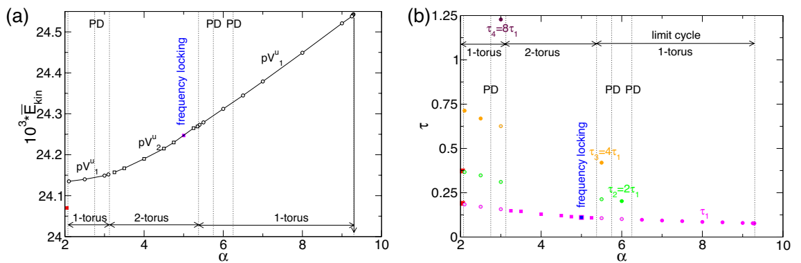
Figure 17. Time dependency of unstable pV^u with \alpha . Variation of (a) E_{kin} and (b) \tau with \alpha for unstable pV^u solutions. PD indicates period-doubling bifurcations. The vertical arrow in (a) illustrates a transition towards the stationary N2 state [outside the presented parameter range (smaller E_{kin} ; see also Fig. 2). Colored symbols in (b) refer to the different period times \tau_i , i \in \{1, 2, 3, 4\} , respectively, which appear throughout the periodic doubling bifurcations (PD) as multiples of the basic period time \tau_i . Thus, these are all 1-torus, that are limit cycle solutions. The filled symbols show the actual period time \tau_p of the corresponding solution, while open symbols illustrate the still underlying time(s) at the bifurcating parameter.
