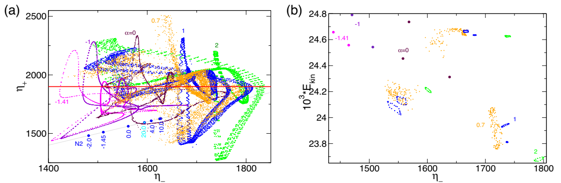
Figure 16. (a) Phase portraits of pV_1 , pV_2 and pV_3 states for \alpha as indicated on (\eta_-, \eta_+) and (b) the corresponding two-dimensional Poincaré sections, (E_{kin}, \eta_-) , with \eta_+ = 1900 (horizontal red line in (a)). Numbers in the figure identify the radial flow, \alpha . The thin gray line in (a) indicates the diagonal \eta_- = \eta_+ , upon which all Z_2 symmetric solutions (i.e., N2) can be found.
