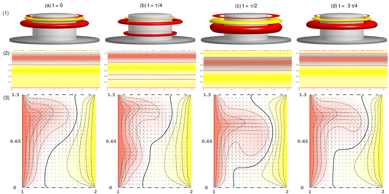
Figure 11. Visualization of the propagating flow state, pV_2 , for \alpha = 2 . As shown in Fig. 9 with isosurfaces of \eta = \pm 240 , the propagation period is \tau_p \approx 0.405 . See also movie, movie_pV2_alpha2.avi , in SMs. Note the clearly visible appearance of the second propagating vortex pair at (b) t = \tau/4 .
