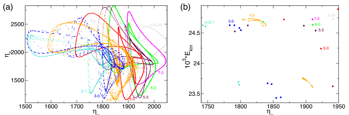
Figure 18. (a) Phase portraits of unstable pV states for \alpha as indicated on (\eta_-, \eta_+) and (b), the corresponding two-dimensional Poincaré sections, (E_{kin}, \eta_-) with \eta_+ = 1900 . Numbers in the figure identify the strength of radial flow, \alpha .
