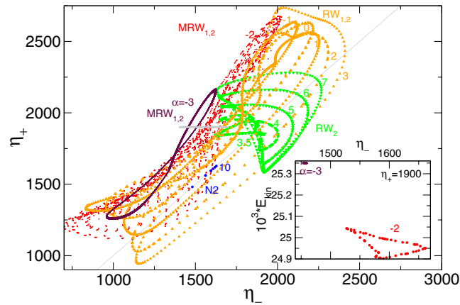
Figure 4. Phase space for rotating flow states. Phase portraits of RW and MRW rotating flow states for \alpha , as indicated on (\eta_-, \eta_+) . The inset shows the corresponding two-dimensional Poincaré section, (E_{kin}, \eta_-) , for \eta_+ = 1900 (horizontal gray line in (\eta_-, \eta_+) ). Numbers in the inset identify corresponding strengths of radial flow \alpha .
