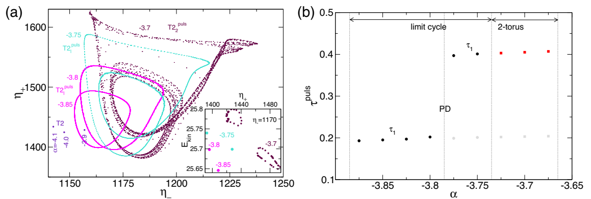
Figure 8. Phase space and period times for T2^{\text{puls}} . (a) Phase portraits of T2_1^{\text{puls}} and T2_2^{\text{puls}} states for \alpha , as indicated on (\eta_-, \eta_+) . The inset shows the corresponding two-dimensional Poincaré sections, (E_{\text{kin}}, \eta_+) , with \eta_- = 1, 170 . (b) Variation with \alpha in time period \tau^{\text{puls}} for T2^{\text{puls}} . Numbers in the figure identify the strength of radial flow, \alpha . Gray-filled symbols highlight the underlying basic period.
