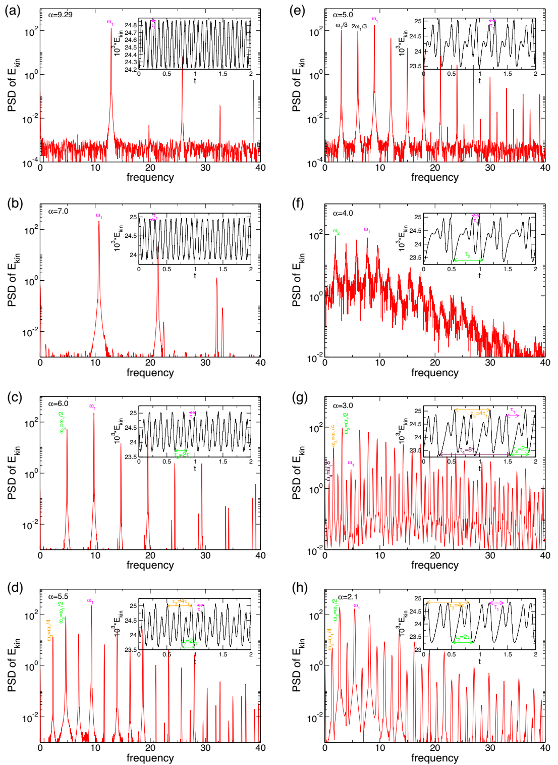
Figure 19. Time series and power spectral densities (PSDs) of E_{kin} of unstably propagating flow states, pV^u , for different \alpha , as indicated. Insets show time series of E_{kin} . In both, dominant times and frequencies, respectively, are highlighted. Note that all PSDy belong to limit cycle solutions (see Fig. 17) but (f) presents a 2-torus solution.
