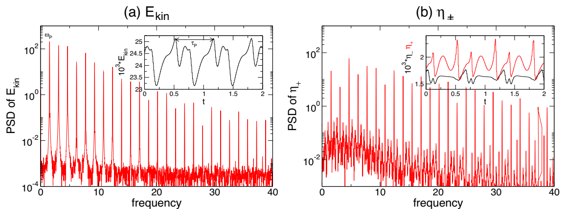
Figure 10. Time series and power spectral densities (PSD) of the pulsating flow state, pV_1 for \alpha = 0 . PSDs of (a) E_{kin} and (b) \eta_+ for the pV_1 state. The propagation/period time (period of vortex generation and annihilation) is \tau_P \approx 0.641 with corresponding frequency \omega_P \approx 1.56 . Insets show time series of E_{kin} , \eta_+ [red], and \eta_- [black].
