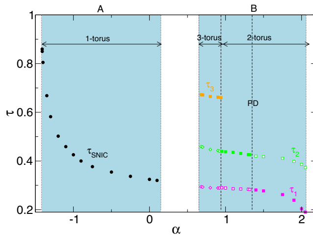
Figure 14. Variation of \tau with radial flow \alpha for stable pV states. Note that in region 0.15 < \alpha < 0.67 , pV s do not appear. Filled symbols highlight the basic period (see PSDs in Fig. 12).
