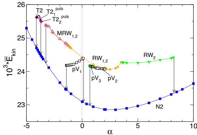
Figure 2. Bifurcation diagram. The total (time-averaged for unsteady flow solutions) modal kinetic energy, \bar{E}_{kin} , as a function of the radial Reynolds number, \alpha . Different flow structures are labeled, and color-coded symbols are used to identify the flow states. Vertical arrows indicate transition behaviors when a flow state loses stability and changes to another stable state. Solid [open] symbols indicate stationary or rotating time dependent solutions.
