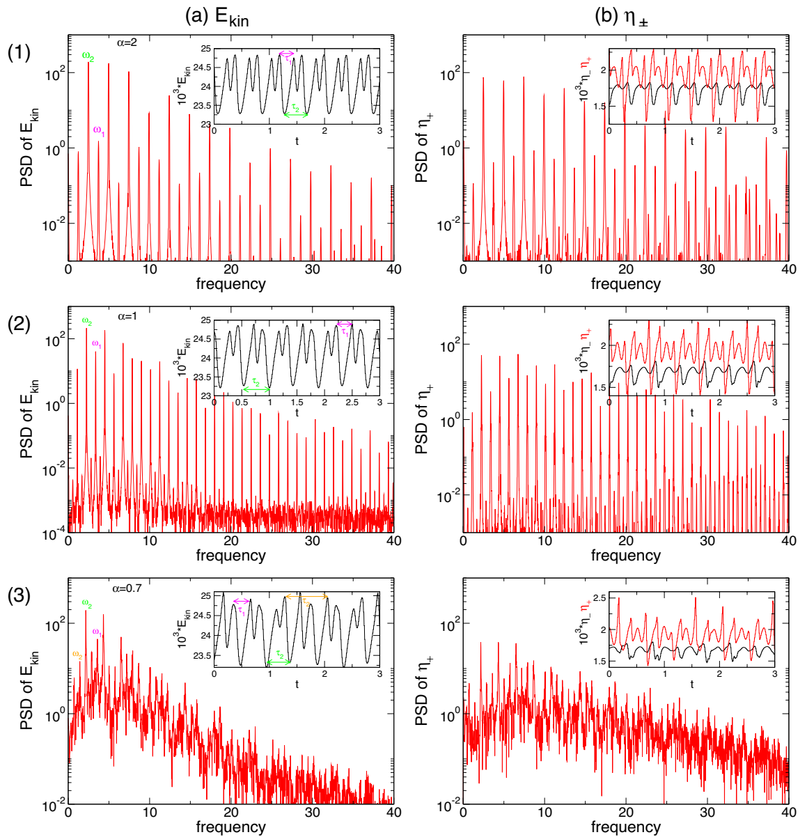
Figure 12. Time series and power spectral densities (PSDs) of pVs for different \alpha . PSDs of (a) E_{kin} and (b) \eta_{\pm} for pVs: (1) \alpha = 2 with period time \tau_p \approx 0.405 and corresponding frequency \omega_p \approx 2.47 ; (2) \alpha = 1 with period time \tau_p \approx 0.896 and corresponding frequency \omega_p \approx 1.116 ; (3) \alpha = 0.7 with period time \tau_p \approx 1.395 and corresponding frequency \omega_p \approx 0.717 . Insets show time series of E_{kin} , \eta_{+} [red], and \eta_{-} [black], respectively.
