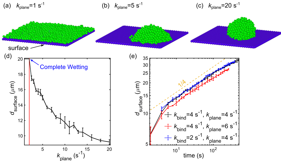
Fig. 6 Colony spreading on planar surfaces. a–c Simulation snapshots of spreading colonies. Depending on the dissociation rate constant of pilus-surface bonds, k_{\text{plane}} , colonies undergo a partial or complete wetting transition. d A complete wetting occurs when k_{\text{plane}} \ll k_{\text{rupt}} = 2 \text{ s}^{-1} . e The time dependence of the diameter of the spreading colony, d_{\text{surface}} , obeys approximately a power law. If not given otherwise, pilus-substrate-binding rates and rupture forces are assumed to be the same as for pilus-pilus bonds, see Table 1. Error bars represent standard deviations from samples of three simulations.
