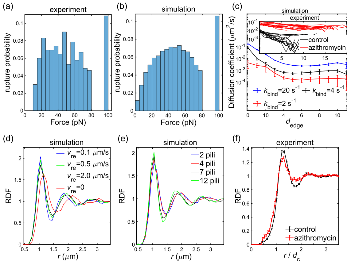
Fig. 3 Pilus-generated forces and local colony order. a Experimental results for the distribution of pilus-pilus bond rupture forces measured with an optical trap 17 . Forces above 80 pN cannot be measured precisely, the histogram bar at 100 pN represents the contribution of all forces over 80 pN. b Distribution of pilus-pilus bond rupture forces in simulations. c Diffusion coefficient of bacteria as a function of distance from the colony edge d_{edge} in simulations. Error bars show standard deviations in three samples. Inset: experimental data for wild-type cells and azithromycin-treated cells 47 . d Radial distribution function (RDF) of cells inside simulated colonies for different pilus retraction velocities. The shape of the functions, with decreasing, quasiperiodic maxima resembles the RDF of a liquid. For passive pili ( v_{re} = 0 ), k_{bind} = 2 \text{ s}^{-1} is used, compare Table 1. e The maxima in the RDF become more pronounced with increasing numbers of pili per cell, thus, pili promote ordering. f Experimentally determined RDF for wild-type cells and azithromycin-treated cells with fewer T4P 47 . The cell diameter d_c is 1.02 \mu\text{m} for the untreated control cells and is 1.42 \mu\text{m} for the azithromycin-treated cells. Error bars are the standard error of the mean with a sample size of 24 colonies.
