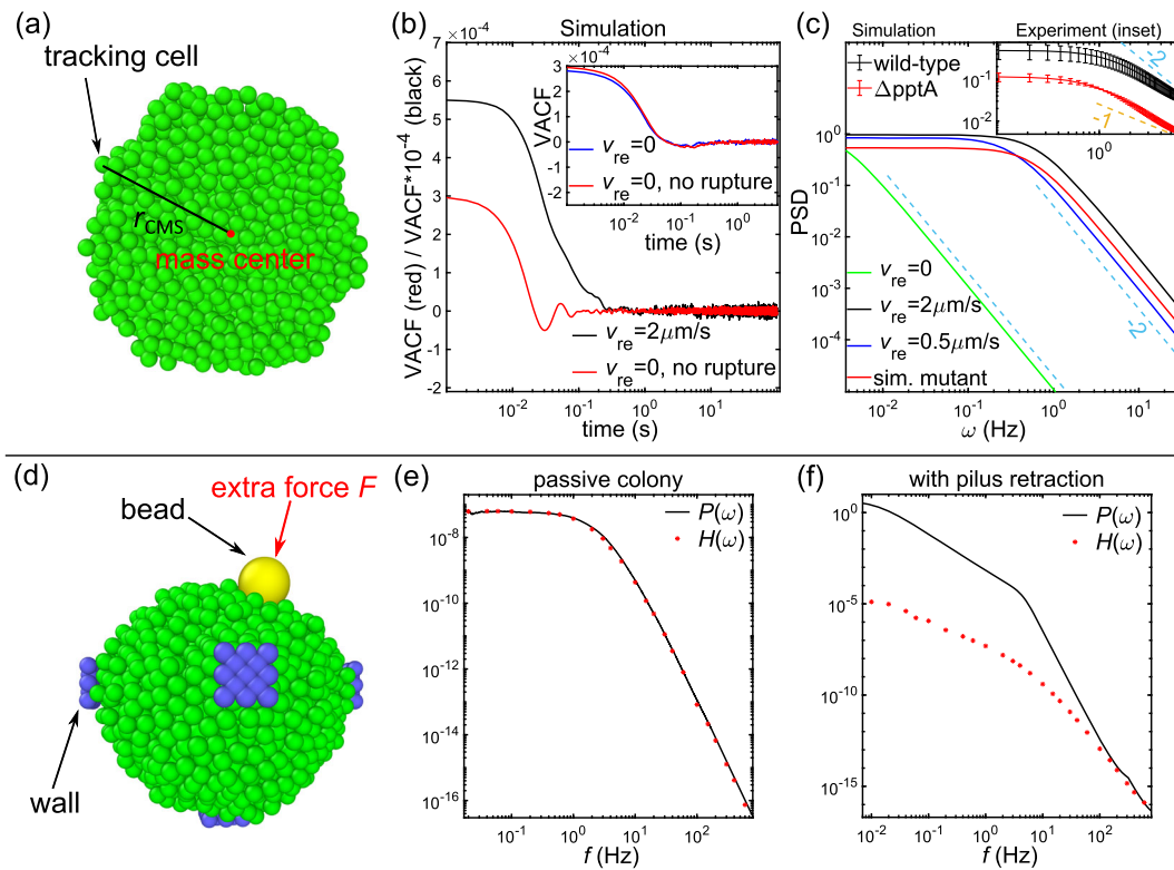
Fig. 5 Active fluctuations at the periphery of colonies. a Simulated setup for quantifying boundary fluctuations by measuring the radial distance r_{\text{CMS}} between a fixed angular position on the surface and the colony center. b Active pilus retraction results in a slower decay of the velocity autocorrelation function (VACF) of the surface point. Main plot: colonies are first grown from cells with retracting pili and the role of pili is studied after growth is switched off. Inset: colonies are grown with retraction-deficient cells. c Active pilus retraction produces a power spectral density of fluctuations characteristic for a visco-elastic material with an elastic behavior at low frequencies. For passive colonies, v_{\text{re}} = 0 , bond rupture results in a viscous material behavior. Colony size is 4000 cells. For comparison with experimental data, a small colony with 600 mutant cells is simulated having a higher binding rate k_{\text{bind}}^{\text{mutant}} = 50 \text{ s}^{-1} , lower rupture rate k_{\text{rupt}}^{\text{mutant}} = 1 \text{ s}^{-1} and lower retraction velocity v_{\text{re}} = 0.5 \mu\text{m/s} . Inset: experimental data for wild-type cells and a \Delta\text{pptA} strain, error bars show standard deviations with three samples. d Simulated setup for colony-shape perturbation. e Simulated mutant colonies with retraction-deficient pili that form permanent bonds. The equilibrium fluctuation-response relationship holds. f For simulated wild-type cells, the equilibrium fluctuation-response relationship is strongly violated ( v_{\text{re}} = 1.0 \mu\text{m/s} , d_{\text{bind}} = 3.0 \mu\text{m} ).
