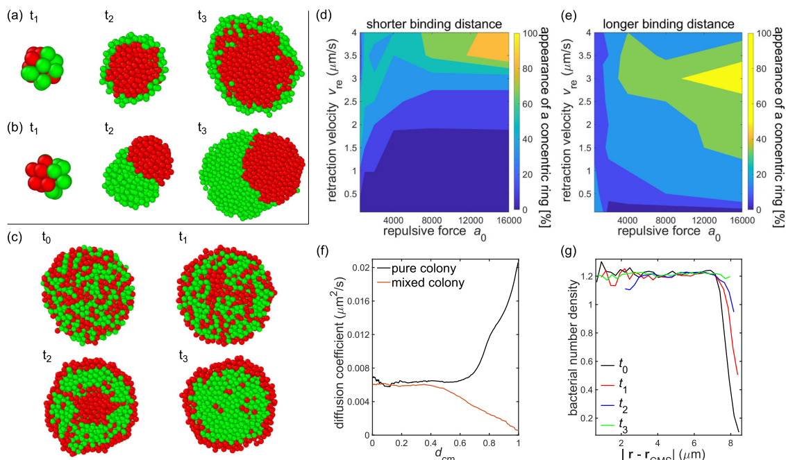
Fig. 4 Phase segregation of mixed colonies. a Simulation snapshots for three time points, t_1 - t_3 , of a growing colony consisting of cells with 14 pili (red) and cells with 7 pili (green). b Snapshots for three time points, t_1 - t_3 , of the simulated growth of a mixture of wild-type cells (WT, green) and mutants deficient in post-translational pilin glycosylation (GD, red) 32 . Pilus rupture forces are as follows: F_{rupt}^{WT-WT} = 22.5 pN, F_{rupt}^{GD-WT} = 20 pN, F_{rupt}^{GD-GD} = 45 pN. In (a) and (b) , Voronoi tessellation is used to locate neighbors for pilus binding. c Segregation of a binary mixture of wild-type bacteria (green) and pilus-retraction-deficient cells (red). Pilus-mediated interactions are long-ranged in this example with d_{bind} = 2.5 \mu\text{m} . At time t_0 , the colony is randomly mixed. Over time, the proportion of pilus-retraction-deficient cells increases in the colony periphery, t_1 , and wild-type cells then accumulate in a concentric sphere inside the colony, t_2 . The concentric sphere eventually disappears and wild-type cells accumulate in the colony center, t_3 . d Lifetime of the concentric sphere arrangement for short-ranged pilus interactions, d_{bind} = 2.5 \mu\text{m} . Lifetimes are given in percent of the longest observed lifetime (3000 s). e Lifetime of the concentric sphere arrangement for long-ranged pilus interactions, d_{bind} = 3.5 \mu\text{m} . Lifetimes are given in percent of 3000 s. f Diffusion coefficients of individual cells as a function of their distance from the colony center divided by the colony radius, d_{cm} . Pure colonies consist of one type of cells, the mixed colony is the segregated system shown in (c) , t_3 . g The mean radial number density of wild-type cells (green) for the simulation snapshots shown in (c) .
