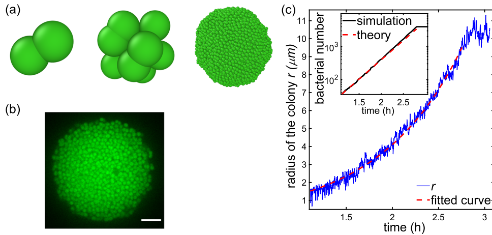
Fig. 2 Simulations of growing colonies. a Simulation snapshots showing colony formation. b Confocal section of a microcolony of fluorescently labeled N. gonorrhoeae . Scale bar: 5 \mu\text{m} . c The colony radii increase exponentially with time during the simulations. Growth and division are switched off before the end of the simulation. Inset: the number of cells increases exponentially with time and simulation results agree with an analytical expression.
