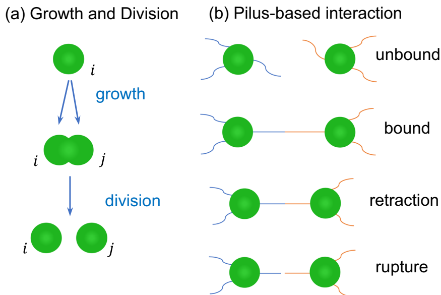
Fig. 1 Schematic representation of the two active processes occurring in the simulations. a A bacterium grows into a diplococcus and then divides into two individual bacteria. b Two cells bind to each other via pili. Subsequently, pili are retracted by the bacteria leading to a force build-up. The bond connecting the pili ruptures stochastically in a force-dependent manner.
