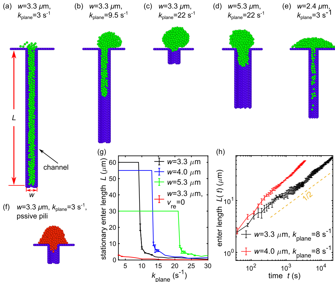
Fig. 7 Colonies atop surfaces containing channels. a–c Simulated wild-type colonies that are initially positioned on top of a narrow channel can invade the channel by making use of pilus activity if the pilus–substrate bonds are strong. The length that a colony enters a channel is denoted by L . d Colonies more easily invade a wider channel. e Invasion of very narrow channels is possible, but colonies break up in this geometry f Passive colonies are not seen to invade channels fully in simulations. g Stationary lengths of colonies after entering channels of different widths. Depending on the channel width, full entrance of the colony occurs below a critical value of k_{\text{plane}} . h The time evolution of the enter length is described approximately by a power law. Error bars represent standard deviations from three simulation samples.
