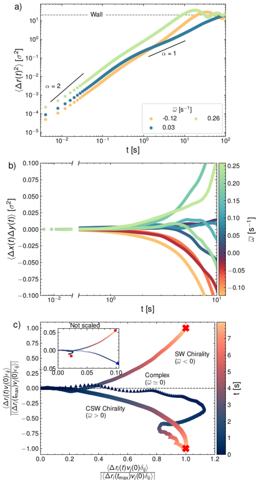
Fig. 1 Statistical properties of particle displacements. a Mean squared displacement \langle \Delta r(t)^2 \rangle at three different global vorticities \bar{\omega} . The saturation value due to confinement is indicated with a dashed line. b Mean cross-displacements \langle \Delta x(t)\Delta y(t) \rangle for several values of \bar{\omega} . c Position-velocity cross correlations for \bar{\omega} = -0.12 \text{ s}^{-1} , \bar{\omega} = 0.03 \text{ s}^{-1} , \bar{\omega} = 0.26 \text{ s}^{-1} (indicated as \bar{\omega} < 0 , \bar{\omega} = 0 , \bar{\omega} > 0 respectively). In the main panel of c , correlations are scaled with the corresponding value at t = t_{\max} = 8 \text{ s} (the last represented value in this case), while in inset shows the unscaled version. Packing fraction for a-c : \phi = 0.45 .
