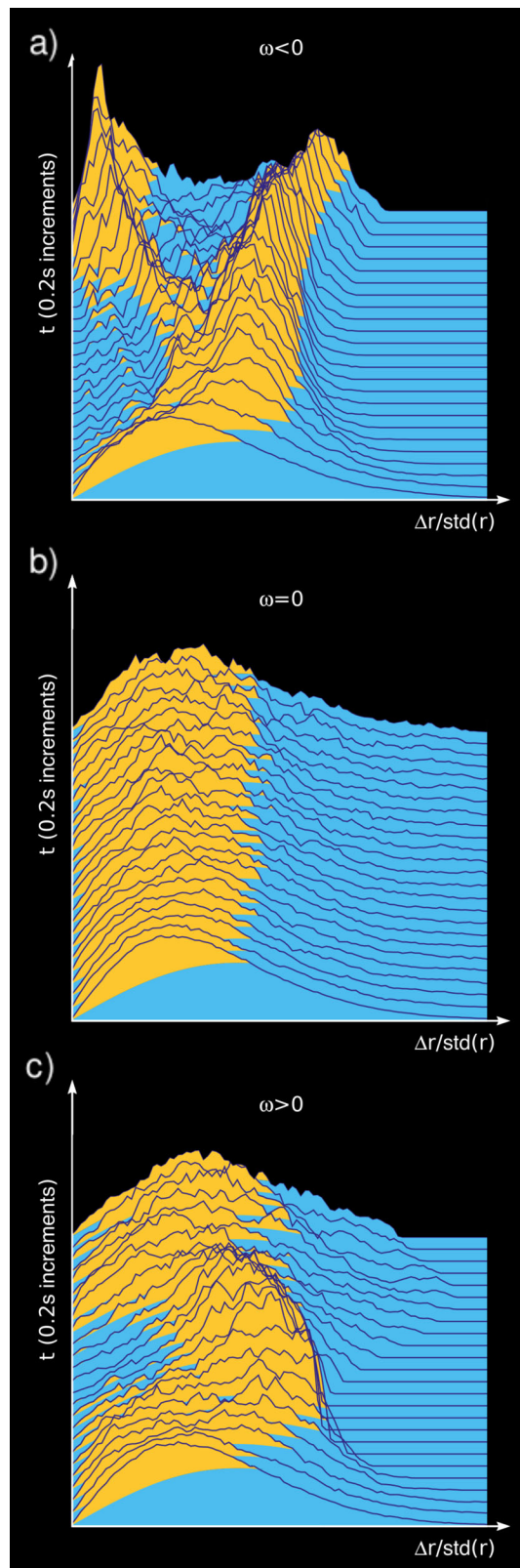
Fig. 2 Time evolution of the distribution function of the root of the reduced square displacements, f(\Delta r/\text{std}(\Delta r)) . We display results for a \bar{\omega} = -0.15 \text{ s}^{-1} , b \bar{\omega} = 0.08 \text{ s}^{-1} and c \bar{\omega} = 0.23 \text{ s}^{-1} (indicated as \bar{\omega} < 0 , \bar{\omega} = 0 , \bar{\omega} > 0 respectively), with packing fraction \phi = 0.45 . Being \text{std}(\Delta r) the standard deviation of \Delta \mathbf{r} . In orange, the areas where f(\Delta r/\text{std}(\Delta r)) > f_G and blue where f(\Delta r/\text{std}(\Delta r)) < f_G (here, f_G is the normal Gaussian distribution).
