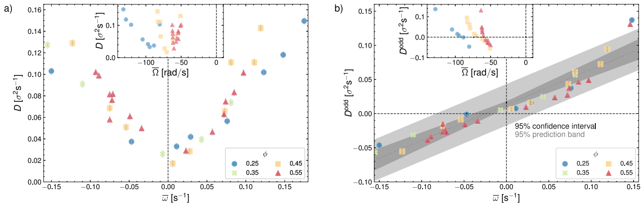
Fig. 3 Diffusion coefficients D , D^{\text{odd}} vs. global mean vorticity \bar{\omega} . Results are represented for several experiments at different densities (each denoted with a different symbol and color, see figure legend). a Diffusion coefficient D (diagonal elements of diffusion tensor \mathcal{D} , in eq. (1)). b Odd diffusion D^{\text{odd}} coefficient (off-diagonal elements of \mathcal{D} ). Confidence intervals of a linear regression from the experimental data for D^{\text{odd}} appear shaded in gray. Insets display diffusion coefficients vs. particle activity (here, average particle spin \bar{\Omega} ). Notice that in the insets D^{\text{odd}} changes sign at different points, contrary to the behavior with respect to the true control parameter \bar{\omega} (main panels).
