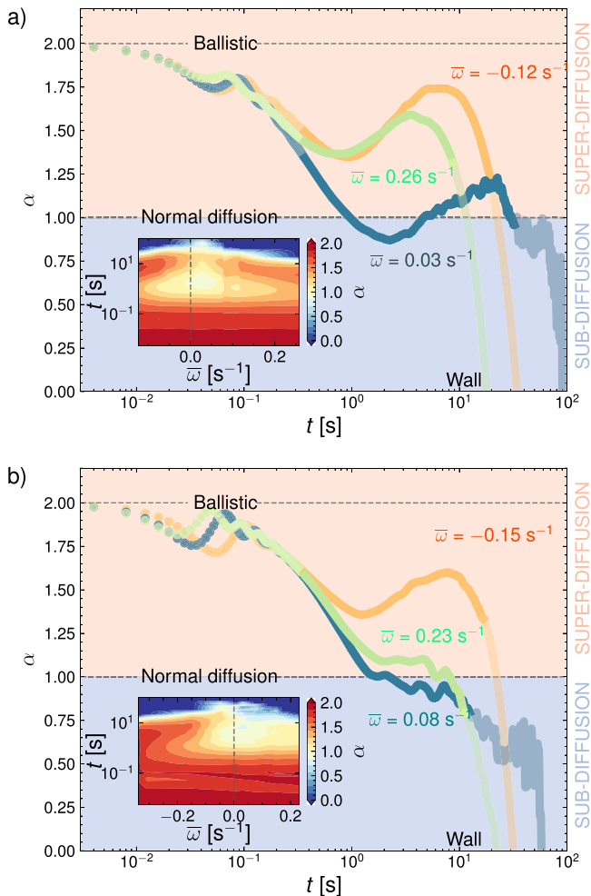
Fig. 4 Evolution of the diffusive exponent \alpha . We show the results for three experiments with \bar{\omega} < 0 , \bar{\omega} = 0 , \bar{\omega} > 0 respectively (each represented in a different color of curve), at two different packing fractions: a \phi = 0.45 and b \phi = 0.25 . Here, t represents lag time. The diffusive exponent has been calculated by performing a rolling fit of the mean squared displacement to a t^\alpha slope. The ballistic regime and normal diffusion regimes are signaled with horizontal lines at \alpha = 2 and \alpha = 1 , respectively. Translucent lines indicate that the system boundary has been reached. Heat-maps in the insets represent \alpha in the \bar{\omega} - t plane (notice the dip at large t , for the case \bar{\omega} \simeq 0 ).
